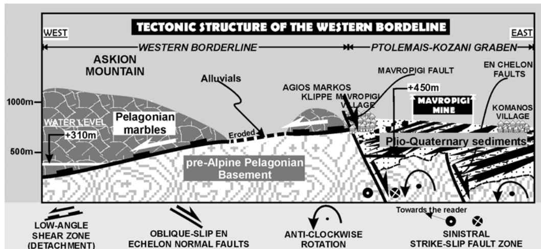
Figure 6. Schematic geological cross-section along the western borderline. It has been noted the westwards tilting of the sediments, the en echelon arrangement of the MSZ, the anti-clockwise rotation of the sediments and also the nappe-structure of the pre-Cretaceous Pelagonian rocks, modified after Diamantopoulos 2003.
